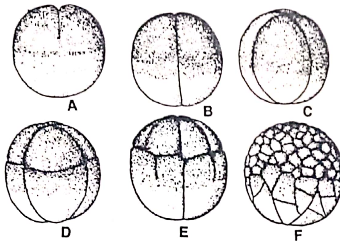
Fig. 2.5. Holoblastic cleavages in Frog egg (Semidiagrammatic)
