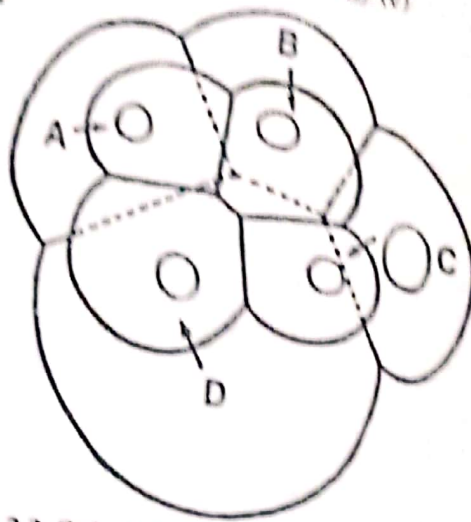
Fig. 2.2. Spiral cleavage in Uta . Blastomere D is larger than A, B, C.
