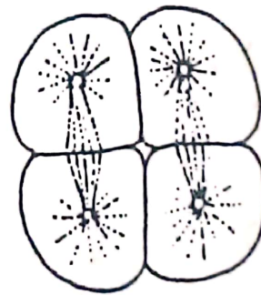
Fig. 2.1. Radial cleavage with equal-sized blastomeres (Viewed from animal pole, 4-cell stage)
