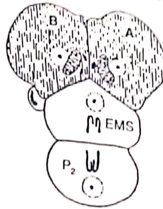
Fig. 2.4. Determinate cleavages in Ascaris
