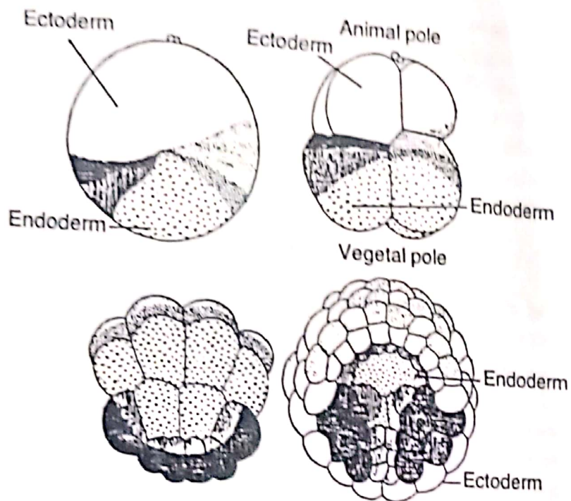
Fig. 2.3. Bilateral cleavages in Ascidian
